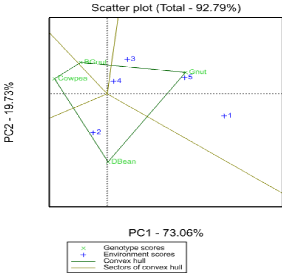
Figure 3: GGE biplot based on environment showing “which-won-where”. The environments are indicated as 1 for Ukulinga 2015/16, 2 for Ukulinga 2016/17, 3 for Umbumbulu 2016/17, 4 for Fountainhill 2015/16 and 5 for Fountainhill 2016/17. Species are denoted by Gnut = groundnut, BGnut = bambara groundnut, DBean = dry bean and cowpea.
