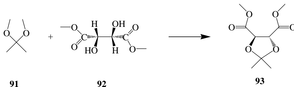
Scheme 19: Synthesis of methyl ester acetone ( 93 )
